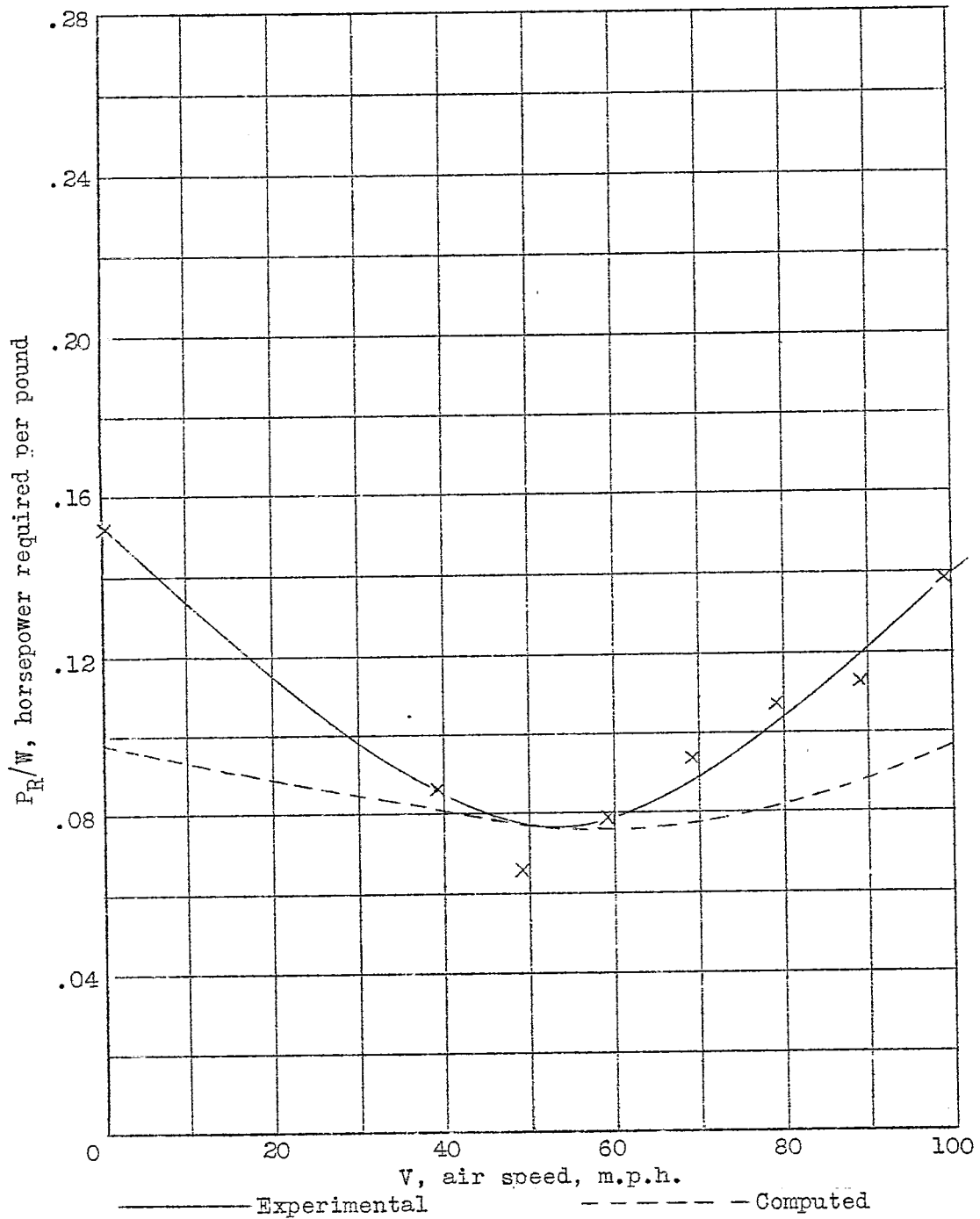
Figure 18.-Cyclogiro performance calculation.
