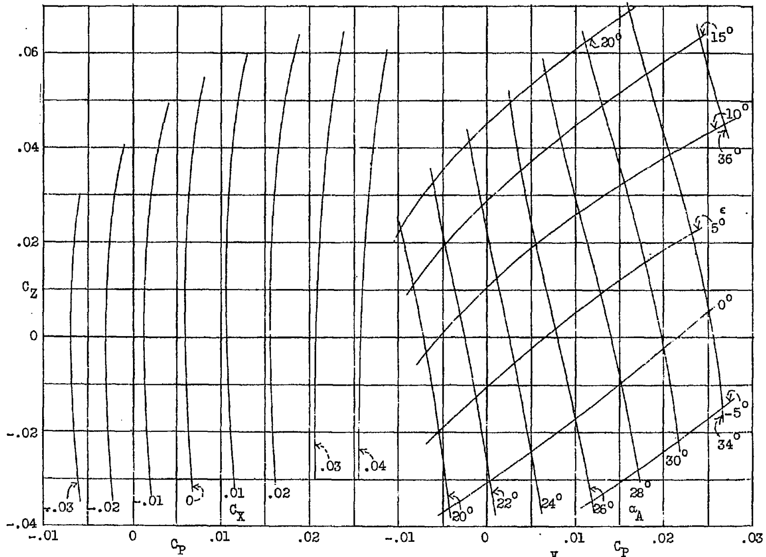
Figure 12.-Level flight. Blades alone; \Omega R = 150 ; \frac{V}{\Omega R} = 0.45
