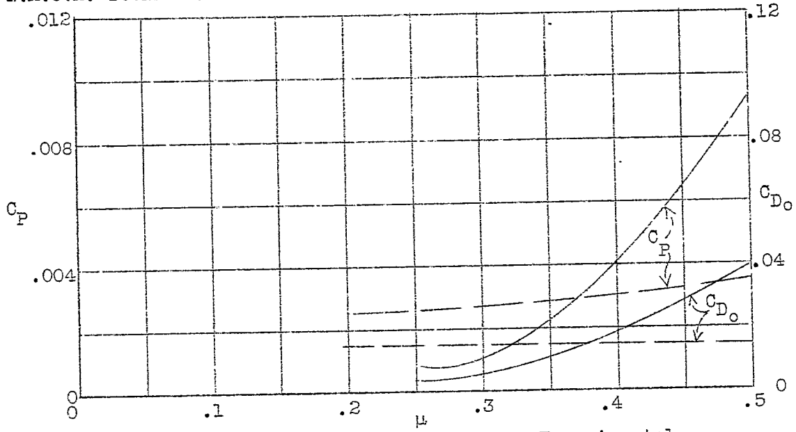
Figure 15.—Comparison of computed and experimental results of C_P and C_{D_0} when C_X and C_Z are zero.
