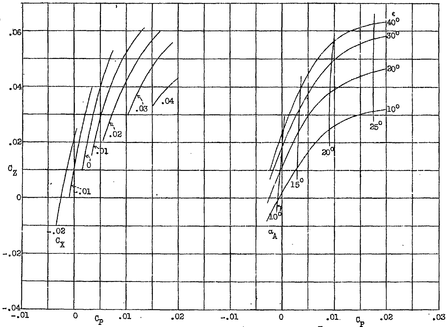
Figure 7.-Level flight. Blades alone; \Omega R = 150 ; \frac{V}{\Omega R} = 0.20
