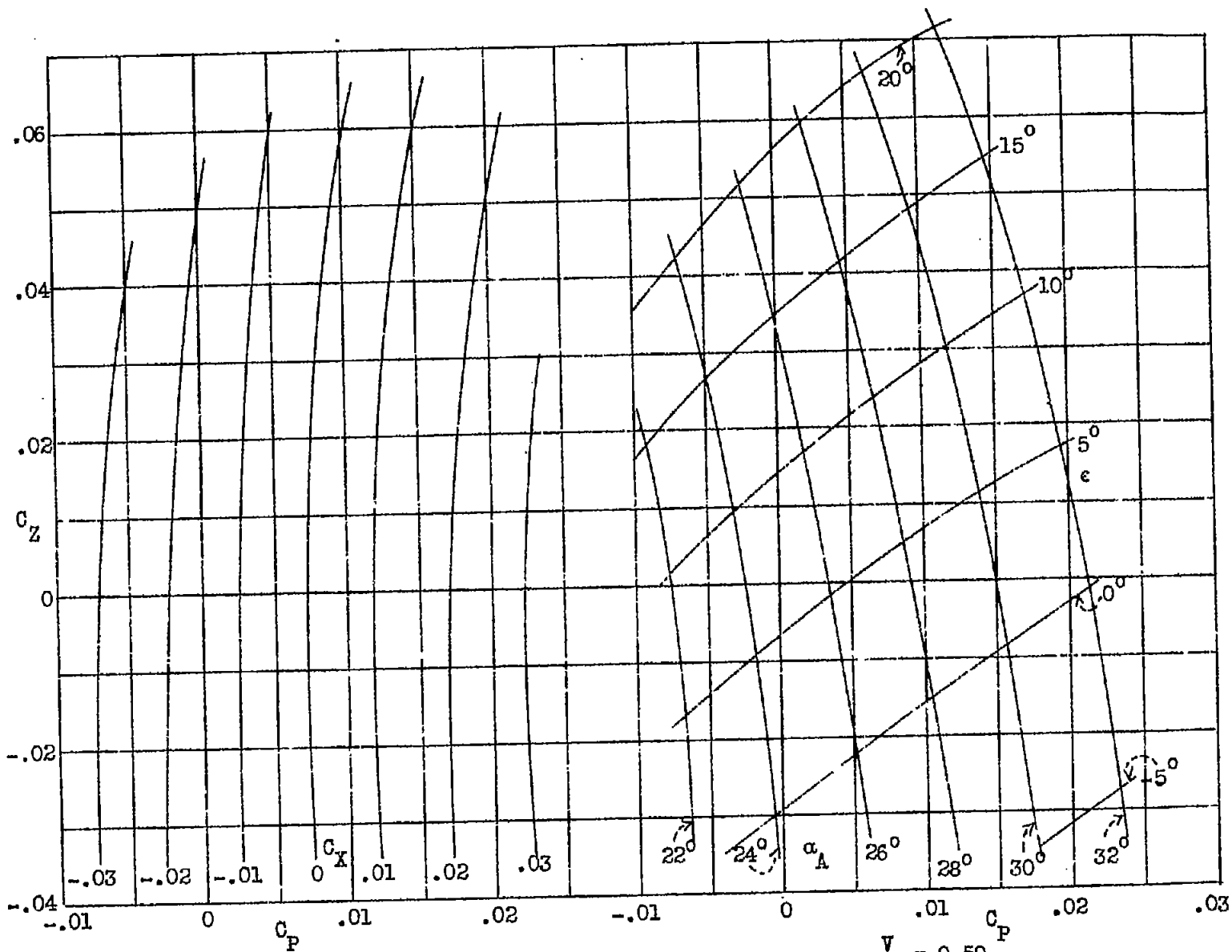
Figure 13.-Level flight. Blades alone; OR = 150 ; \frac{V}{OR} = 0.50
